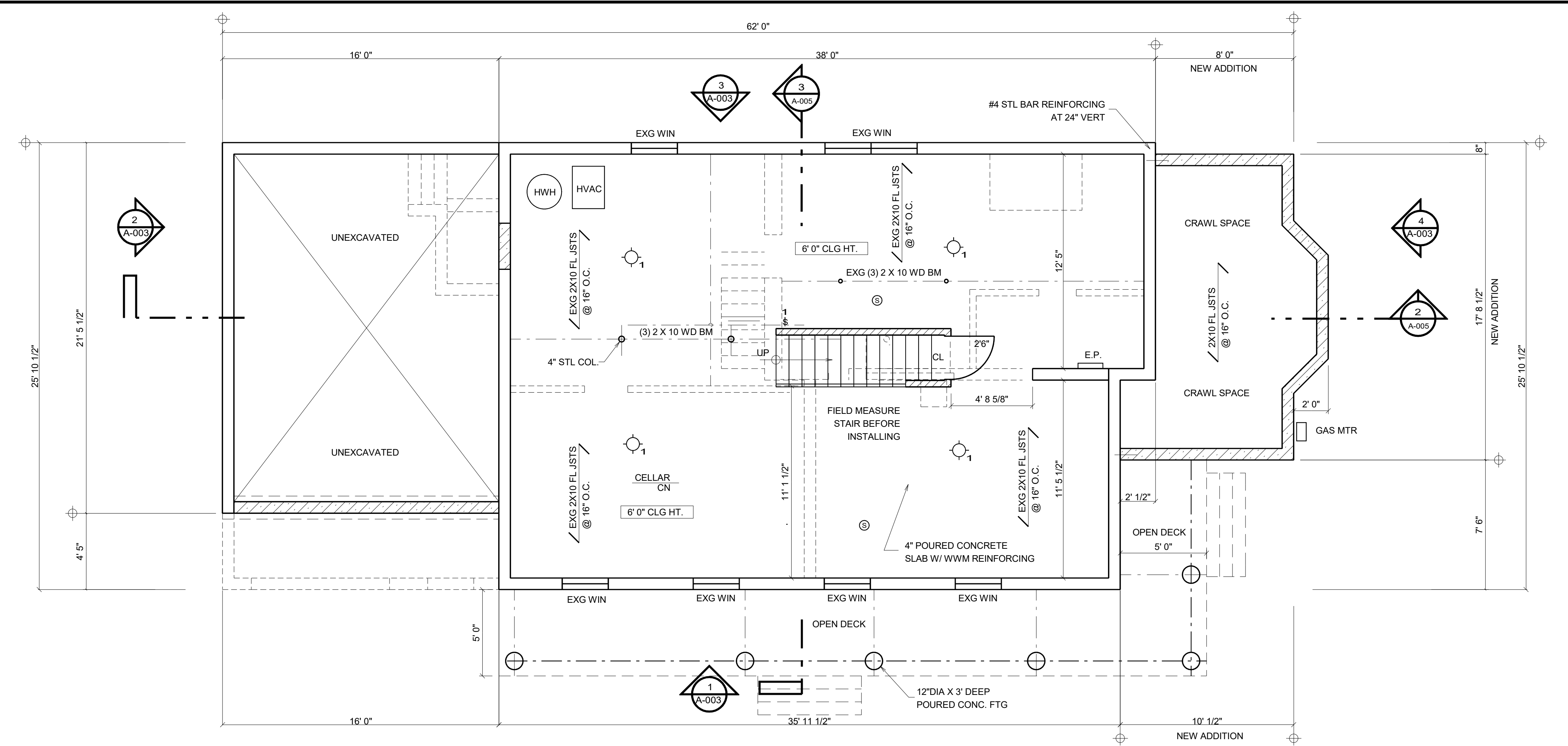
1 CELLAR FLOOR PLAN
