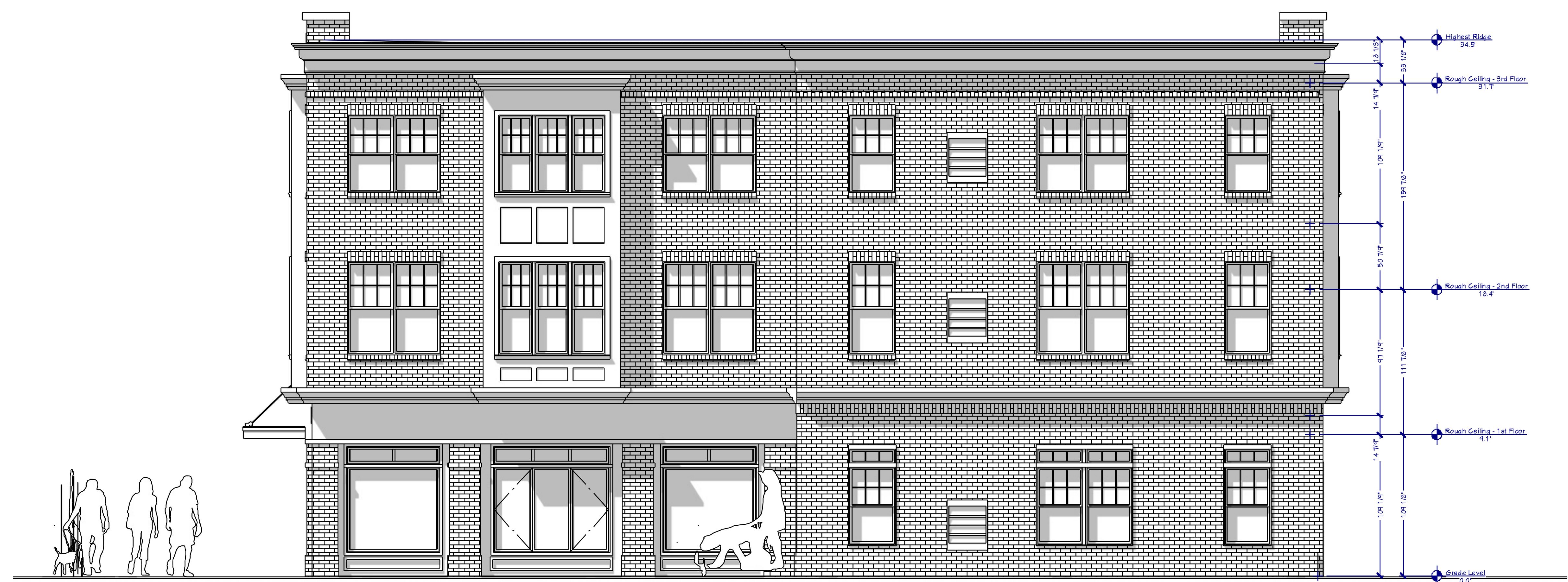
FRONT ELEVATION (CENTRAL AVE) 1/4 in = 1 ft
