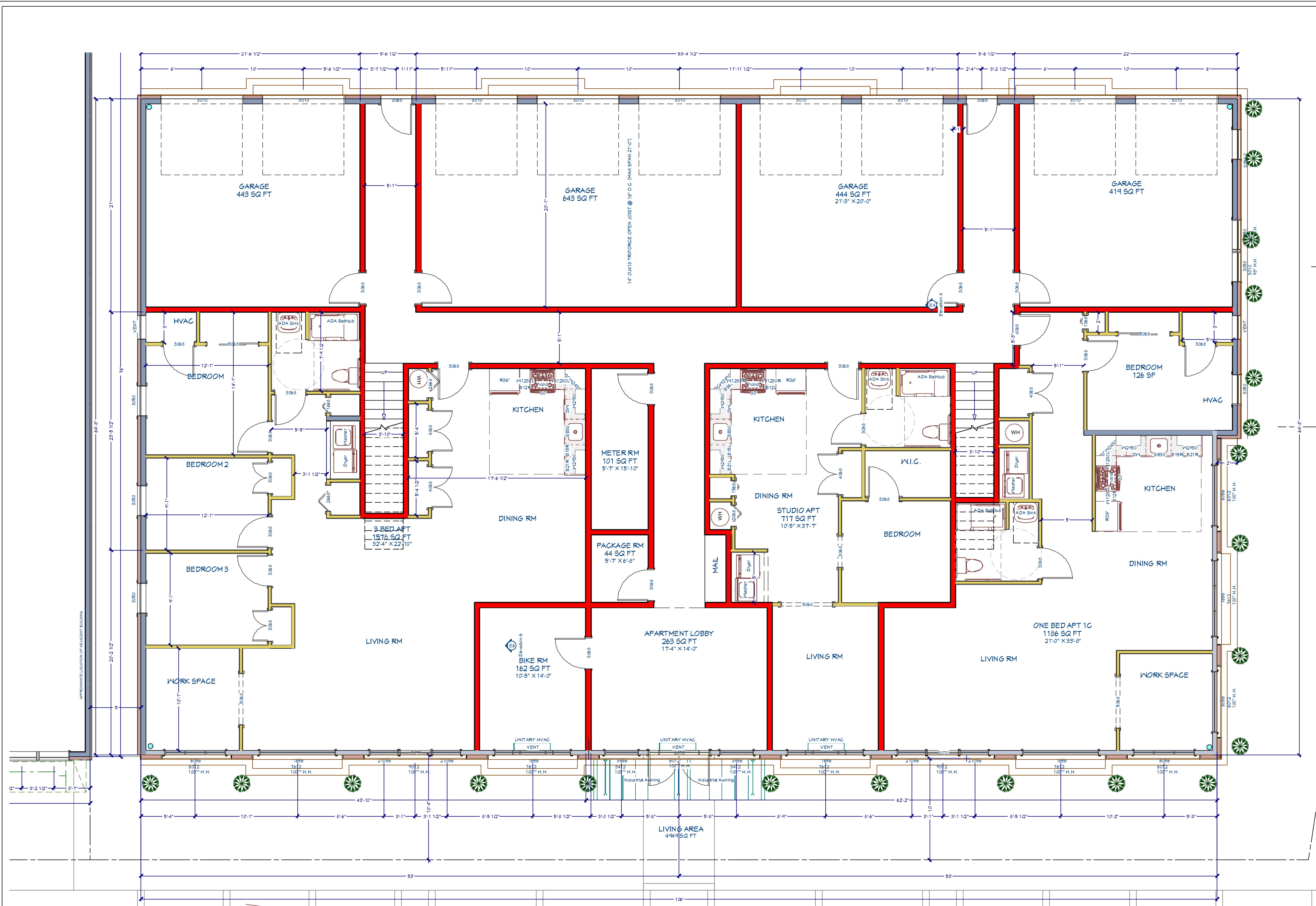
1st Floor 1/4 in = 1 ft
